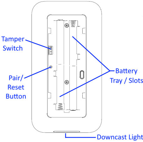
Keypad (back view, open; battery cover / mounting plate off) —
